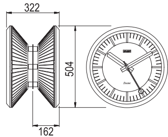
Profil TGV 950 single or double face
