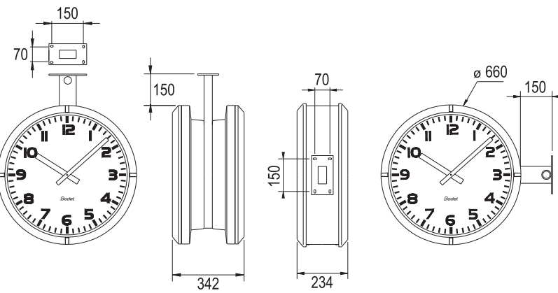
Profil 960 single or double face
