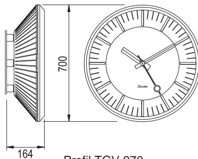
Profil TGV 970 single or double face
