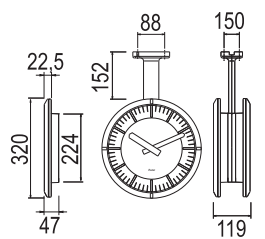
Profil TGV 930 single or double face
